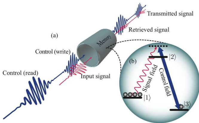
Fig. 8. (a) A Raman memory. The signal is directed into the memory along with a bright write pulse and is stored. If the storage is partial, any unstored signal is transmitted through the memory. A subsequent read pulse extracts the stored excitation, which emerges along with the transmitted read pulse. (b) The \Lambda -level structure of the atoms in the memory. The atoms are prepared in the ground state |1\rangle by optical pumping. The signal is tuned into two-photon resonance with the control field; both are detuned from the excited state |2\rangle . Absorption of a signal photon transfers an atom from |1\rangle into the storage state |3\rangle via Raman scattering stimulated by the control. Upon retrieval the interaction is reversed.
